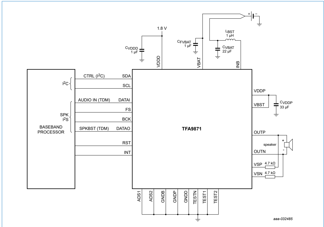
Figure 12-1: Typical mono application
