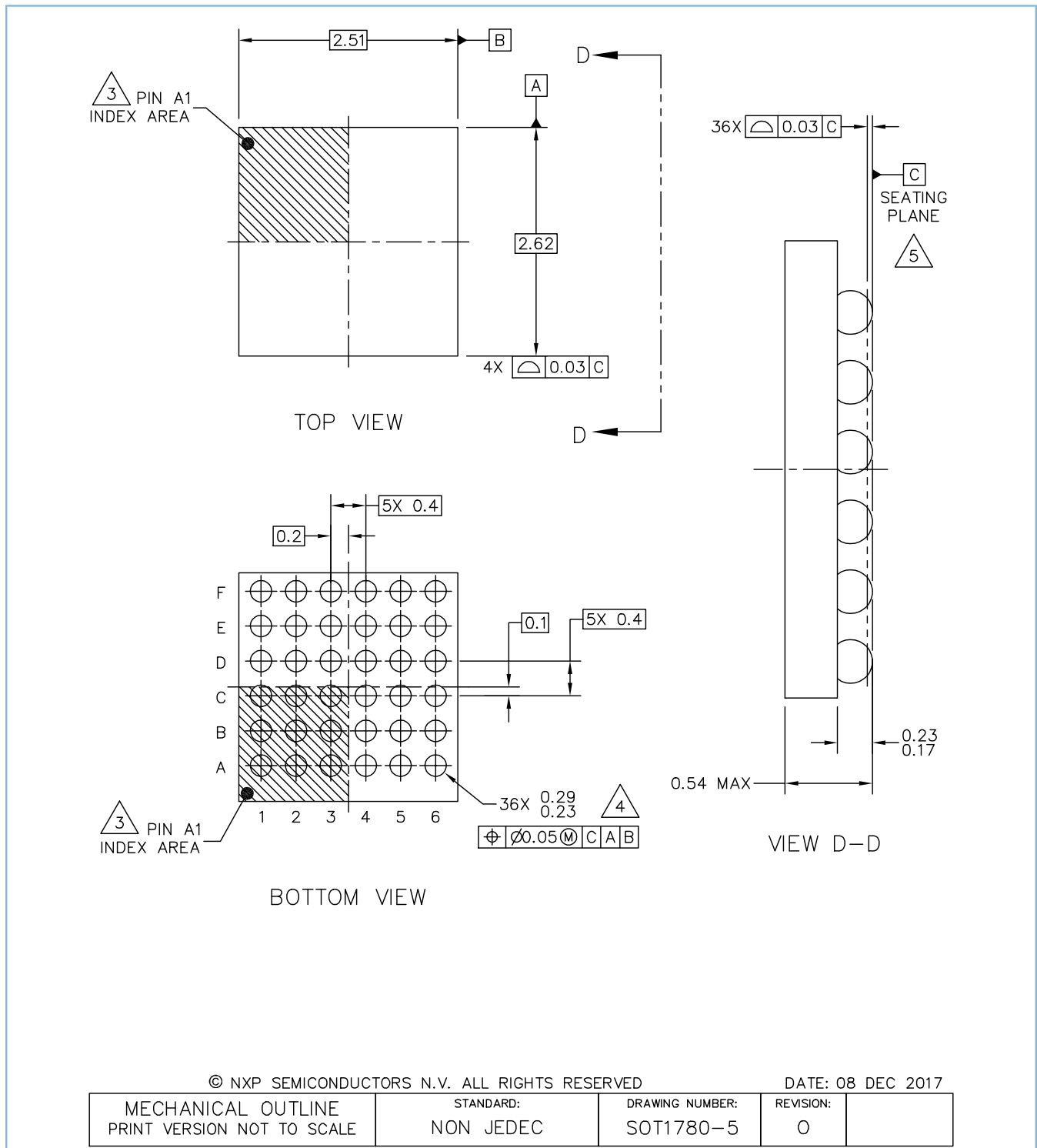
Figure 13-1: Package outline WLCSP36 (SOT1780-5); no back side coating
